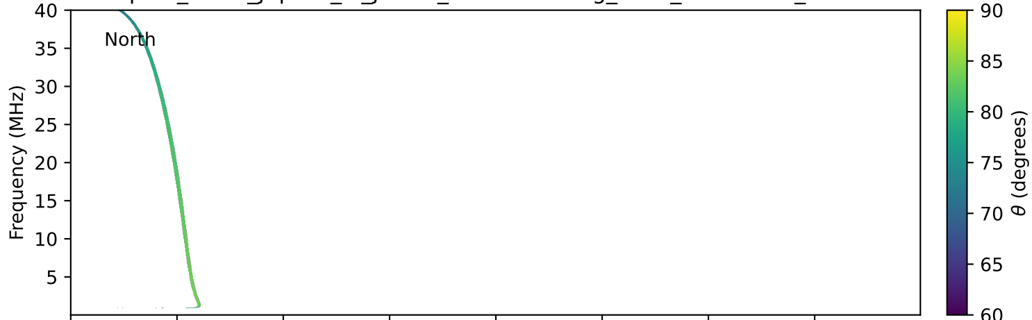
expres_earth_jupiter_io_jrm33_lossc-wid1deg_3kev_20030607_v11.cdf
