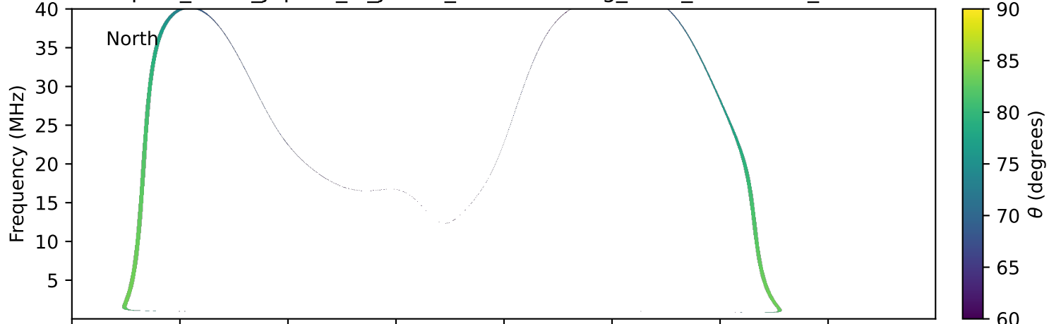
expres_earth_jupiter_io_jrm33_lossc-wid1deg_3kev_20030601_v11.cdf
