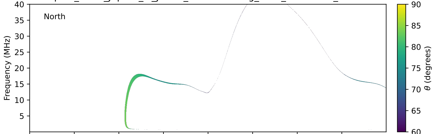
expres_earth_jupiter_io_jrm09_lossc-wid1deg_3kev_20030622_v11.cdf
