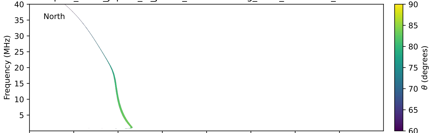
expres_earth_jupiter_io_jrm09_lossc-wid1deg_3kev_20030621_v11.cdf
