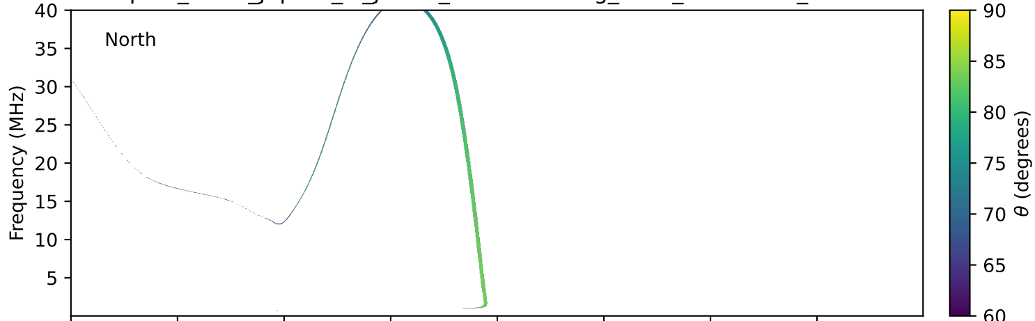
expres_earth_jupiter_io_jrm09_lossc-wid1deg_3kev_20030612_v11.cdf
