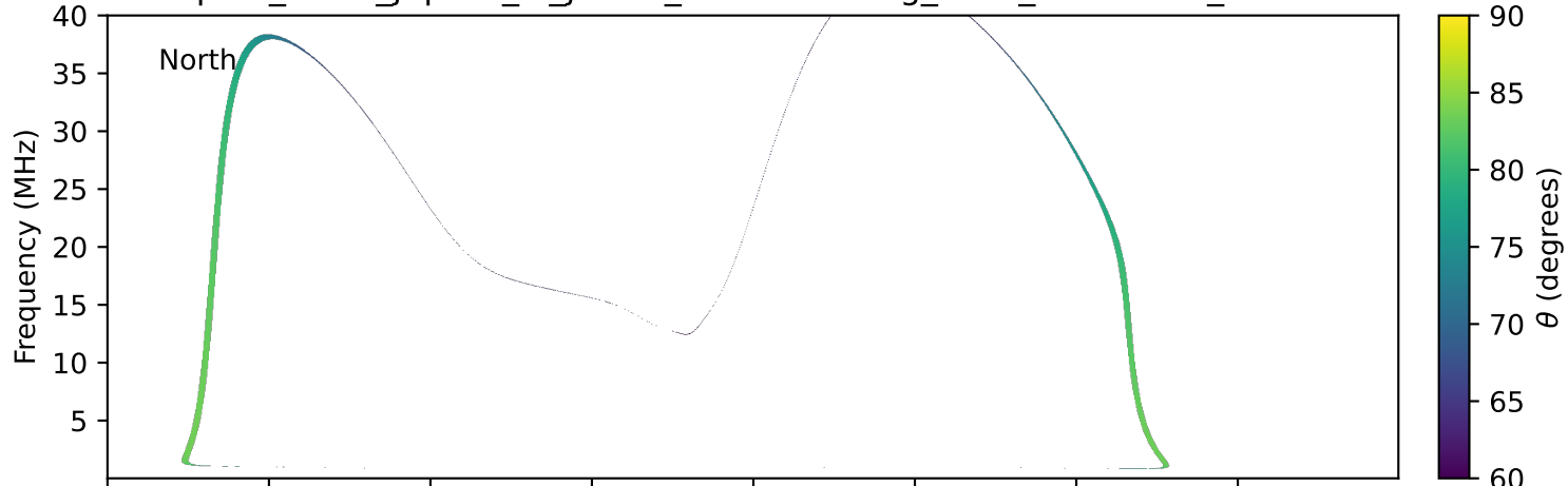
expres_earth_jupiter_io_jrm09_lossc-wid1deg_3kev_20030601_v11.cdf
