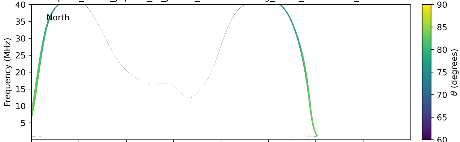
expres_earth_jupiter_io_jrm33_lossc-wid1deg_3kev_20030525_v11.cdf
