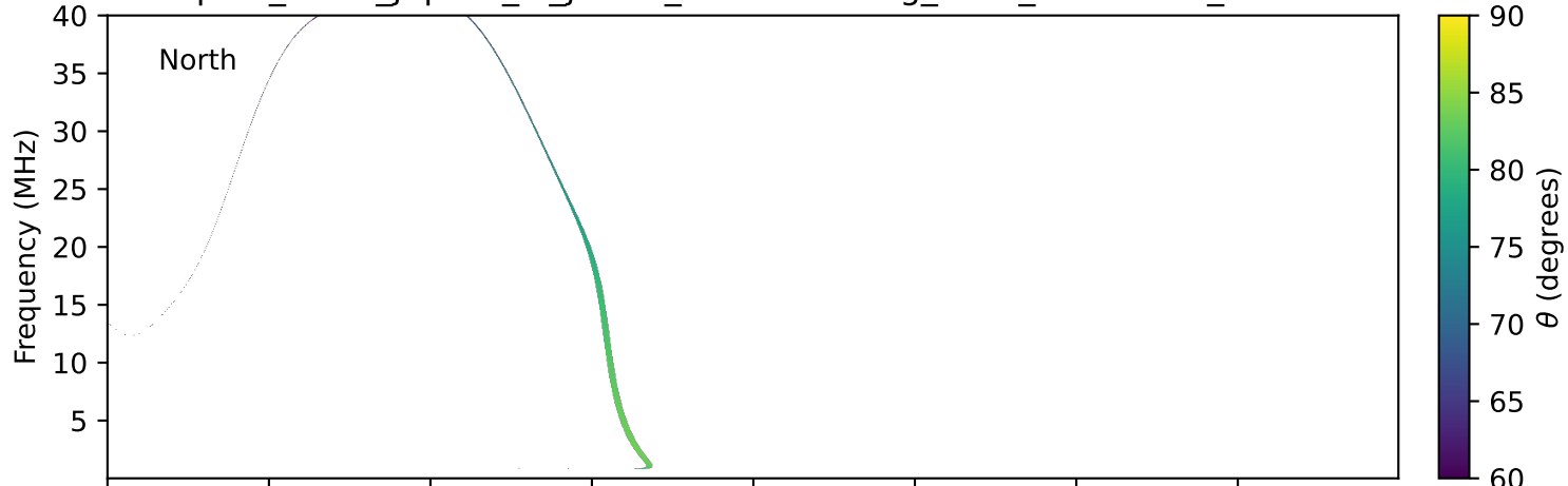
expres_earth_jupiter_io_jrm33_lossc-wid1deg_3kev_20030520_v11.cdf
