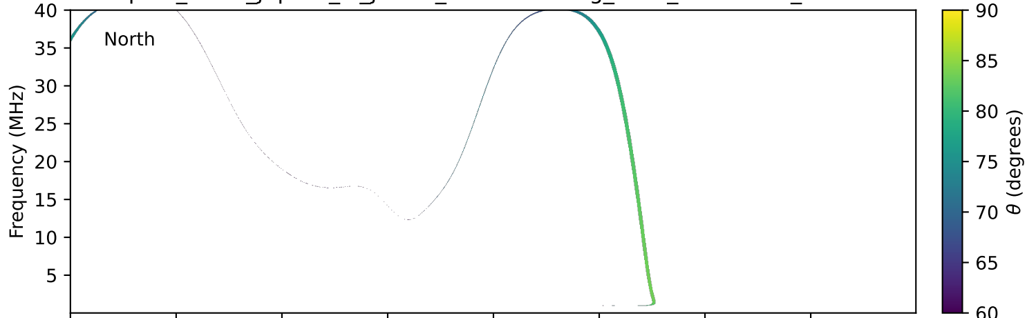
expres_earth_jupiter_io_jrm33_lossc-wid1deg_3kev_20030518_v11.cdf
