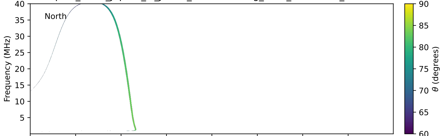
expres_earth_jupiter_io_jrm33_lossc-wid1deg_3kev_20030506_v11.cdf
