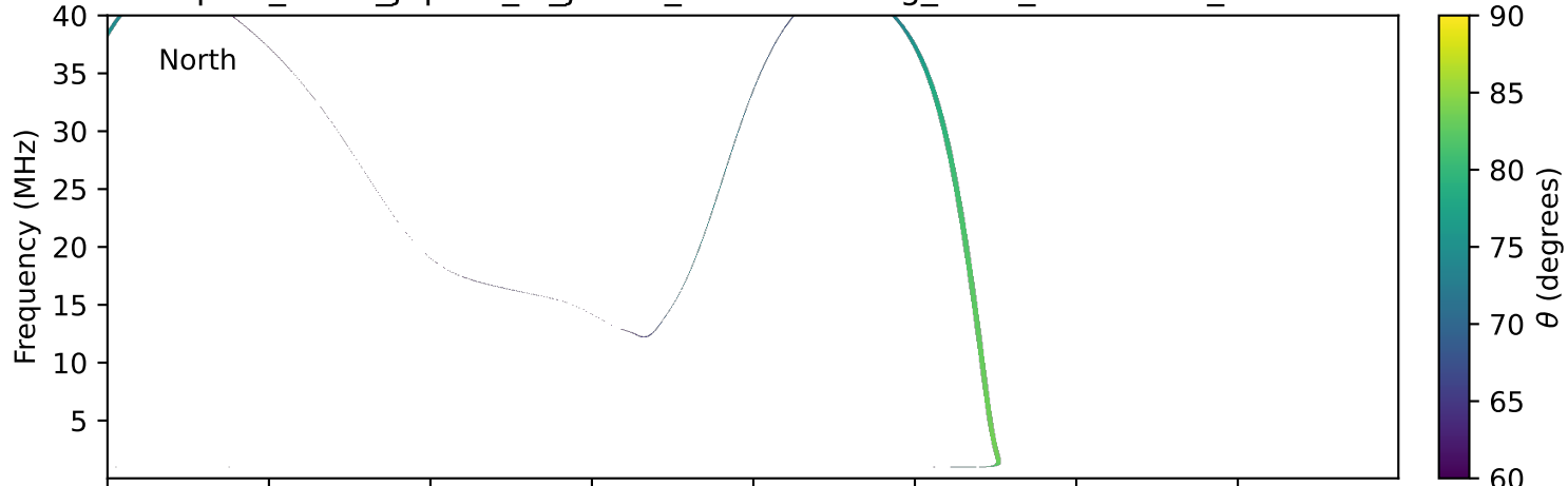
expres_earth_jupiter_io_jrm09_lossc-wid1deg_3kev_20030518_v11.cdf
