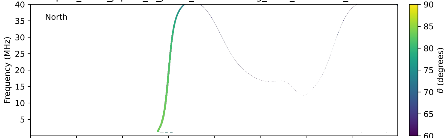
expres_earth_jupiter_io_jrm33_lossc-wid1deg_3kev_20030329_v11.cdf
