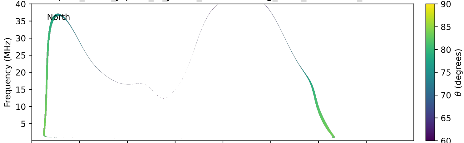
expres_earth_jupiter_io_jrm33_lossc-wid1deg_3kev_20030324_v11.cdf
