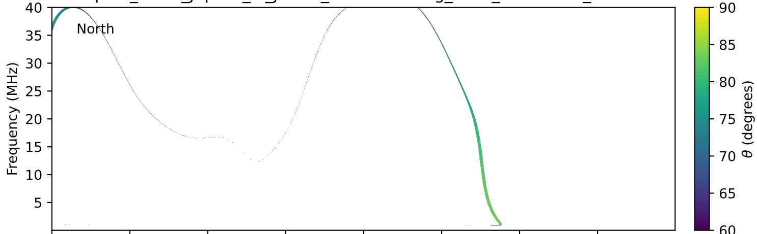
expres_earth_jupiter_io_jrm33_lossc-wid1deg_3kev_20030317_v11.cdf
