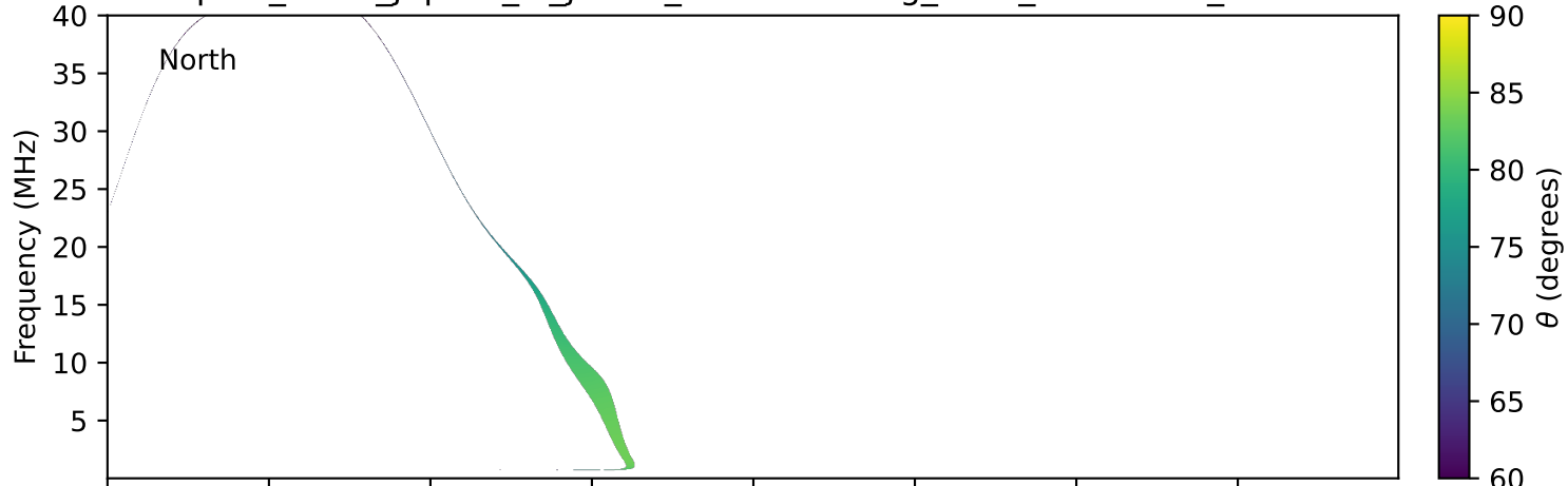
expres_earth_jupiter_io_jrm33_lossc-wid1deg_3kev_20030312_v11.cdf
