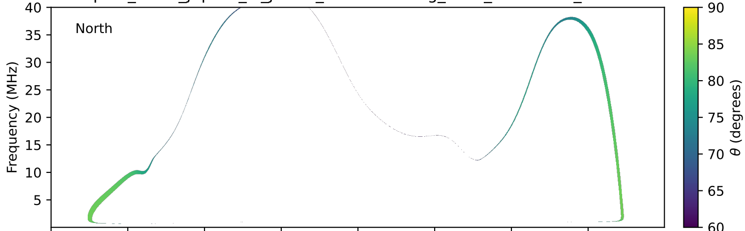
expres_earth_jupiter_io_jrm33_lossc-wid1deg_3kev_20030308_v11.cdf
