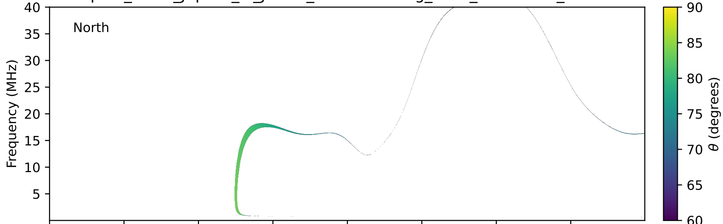
expres_earth_jupiter_io_jrm33_lossc-wid1deg_3kev_20030306_v11.cdf
