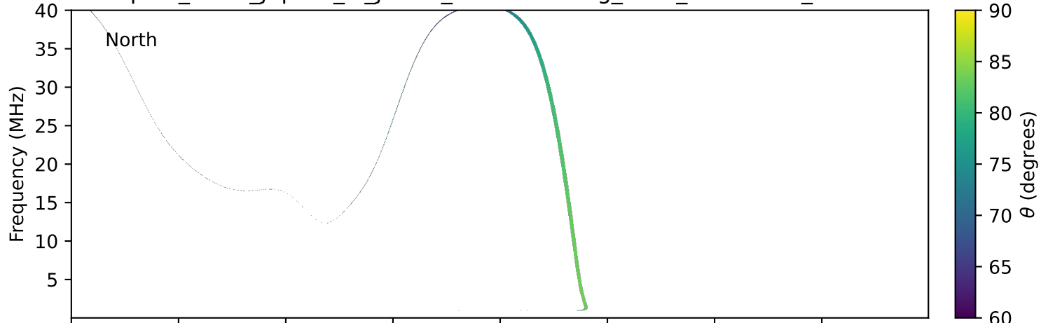
expres_earth_jupiter_io_jrm33_lossc-wid1deg_3kev_20030303_v11.cdf
