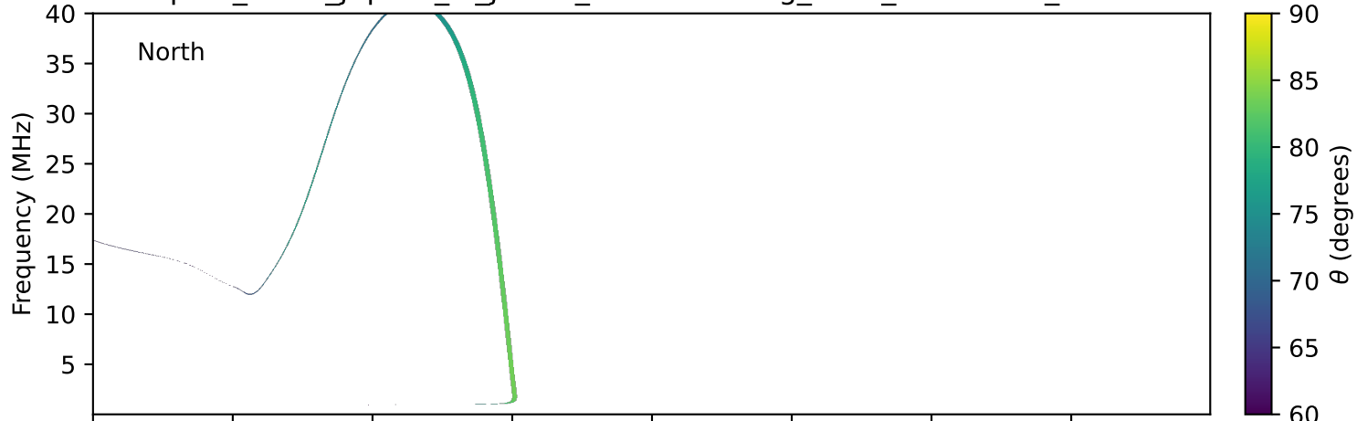
expres_earth_jupiter_io_jrm09_lossc-wid1deg_3kev_20030328_v11.cdf
