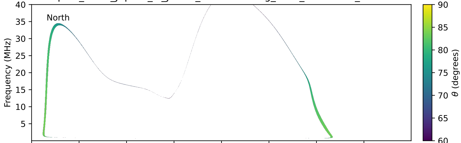
expres_earth_jupiter_io_jrm09_lossc-wid1deg_3kev_20030324_v11.cdf
