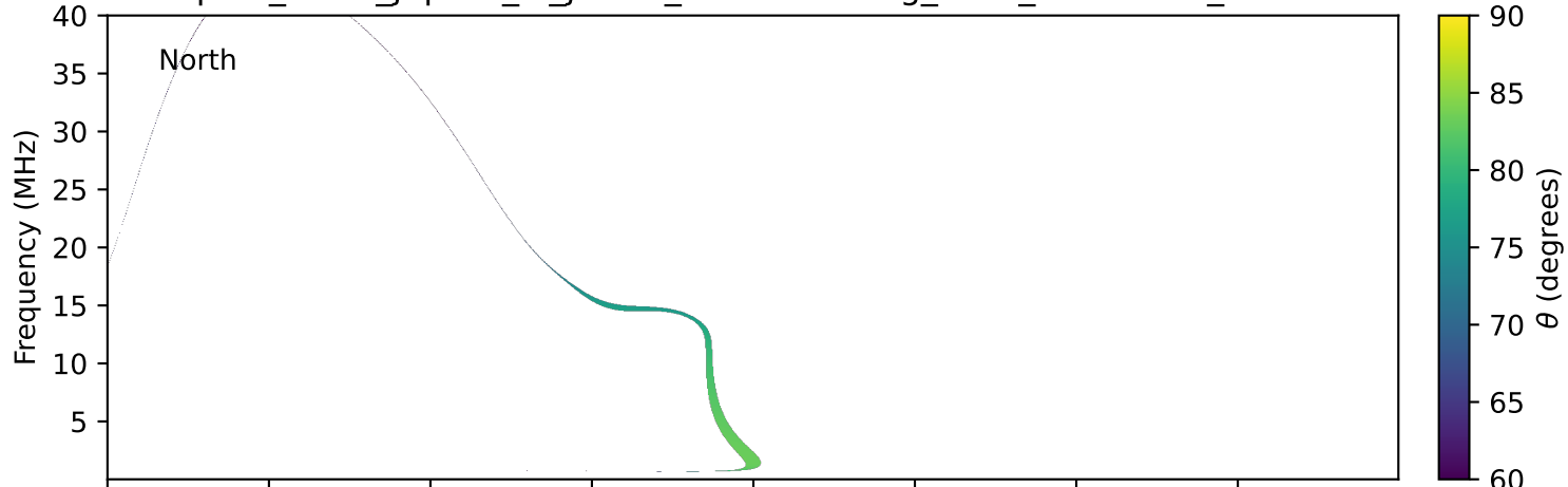
expres_earth_jupiter_io_jrm09_lossc-wid1deg_3kev_20030319_v11.cdf
