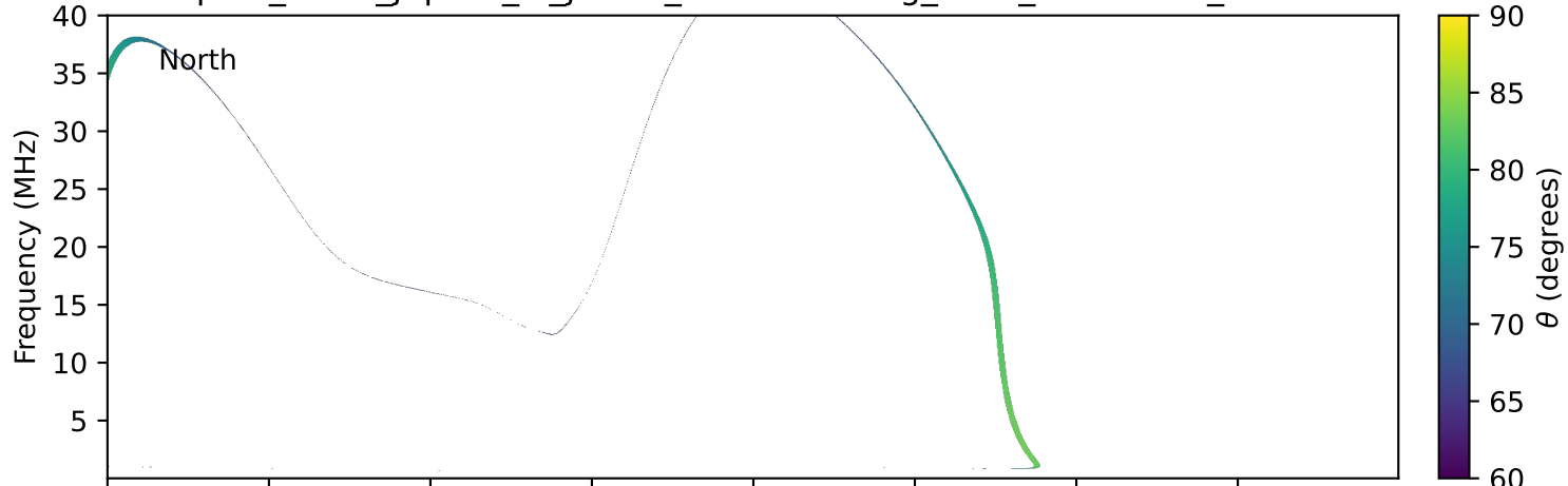
expres_earth_jupiter_io_jrm09_lossc-wid1deg_3kev_20030317_v11.cdf
