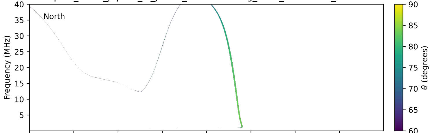
expres_earth_jupiter_io_jrm09_lossc-wid1deg_3kev_20030303_v11.cdf
