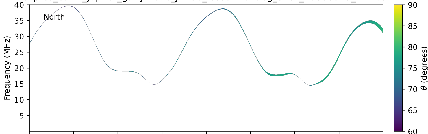
expres_earth_jupiter_ganymede_jrm33_lossc-wid1deg_3kev_20030329_v11.cdf
