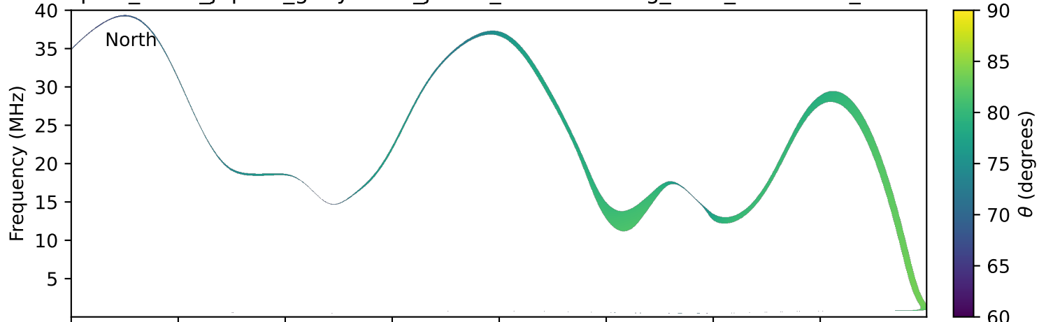
expres_earth_jupiter_ganymede_jrm33_lossc-wid1deg_3kev_20030315_v11.cdf
