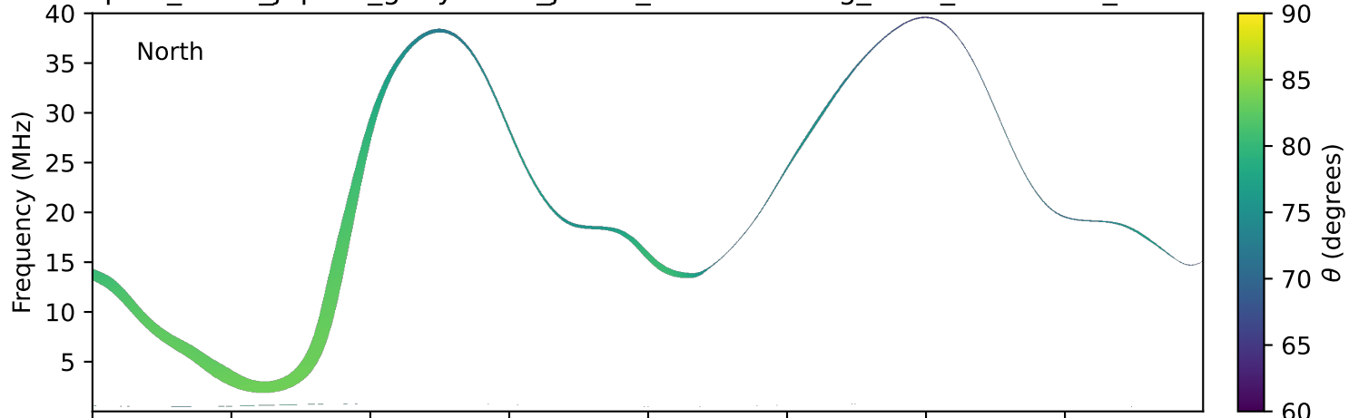
expres_earth_jupiter_ganymede_jrm33_lossc-wid1deg_3kev_20030313_v11.cdf
