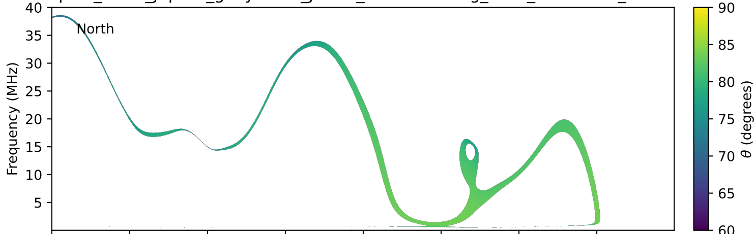
expres_earth_jupiter_ganymede_jrm33_lossc-wid1deg_3kev_20030301_v11.cdf
