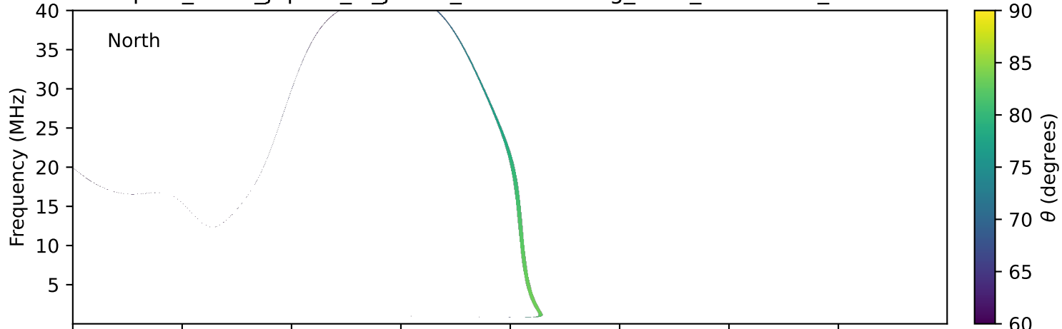
expres_earth_jupiter_io_jrm33_lossc-wid1deg_3kev_20011228_v11.cdf
