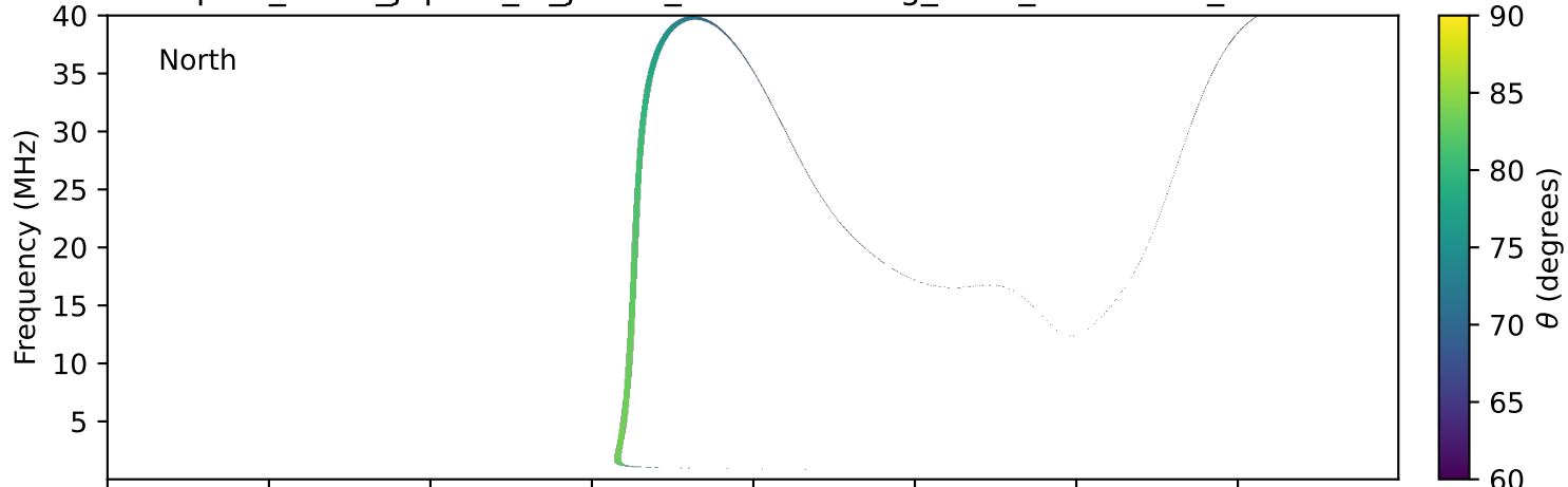
expres_earth_jupiter_io_jrm33_lossc-wid1deg_3kev_20011215_v11.cdf
