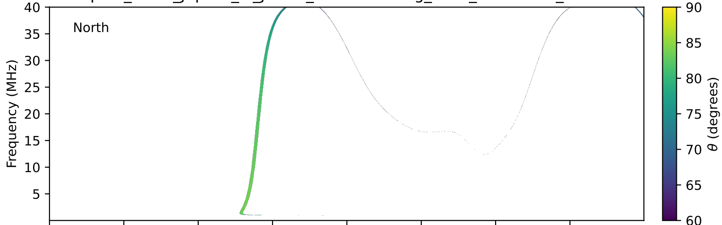
expres_earth_jupiter_io_jrm33_lossc-wid1deg_3kev_20011208_v11.cdf
