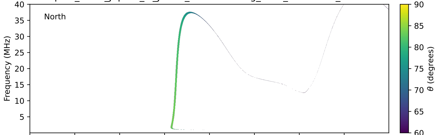
expres_earth_jupiter_io_jrm09_lossc-wid1deg_3kev_20011215_v11.cdf
