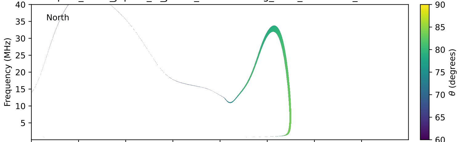
expres_earth_jupiter_io_jrm09_lossc-wid1deg_3kev_20011212_v11.cdf
