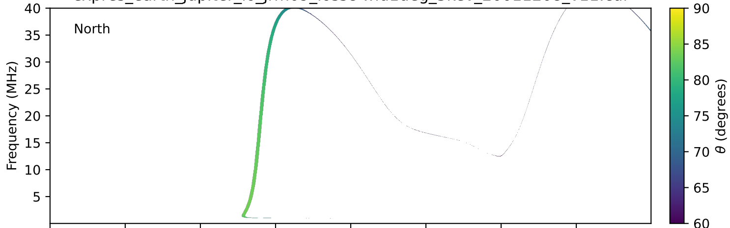
expres_earth_jupiter_io_jrm09_lossc-wid1deg_3kev_20011208_v11.cdf
