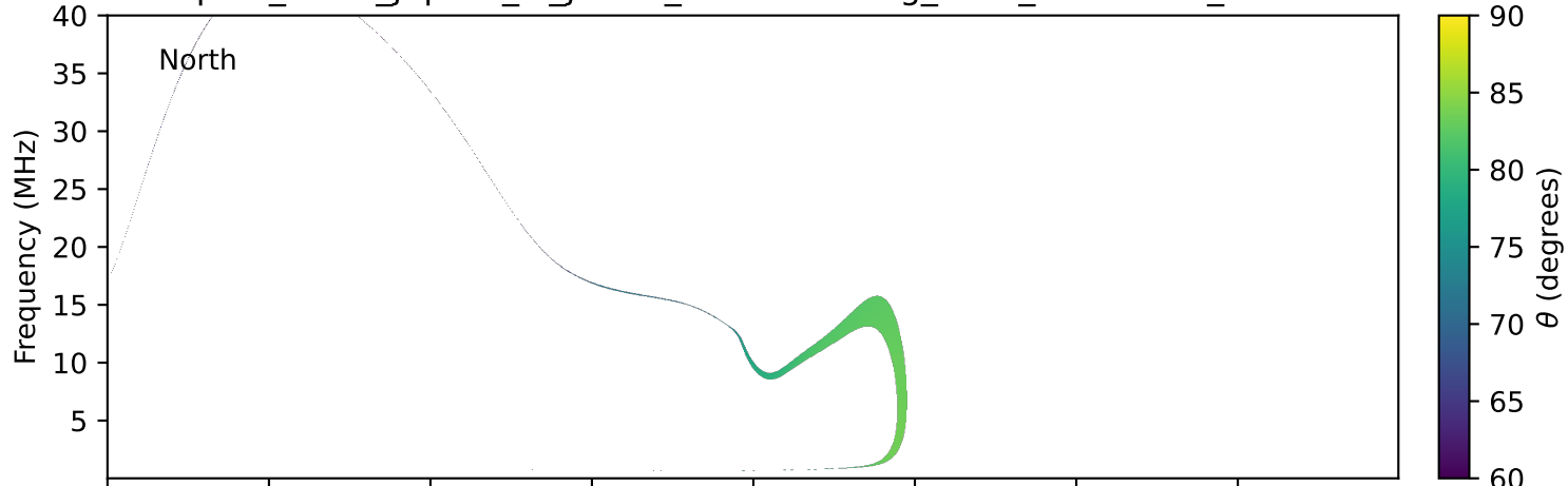
expres_earth_jupiter_io_jrm09_lossc-wid1deg_3kev_20011205_v11.cdf
