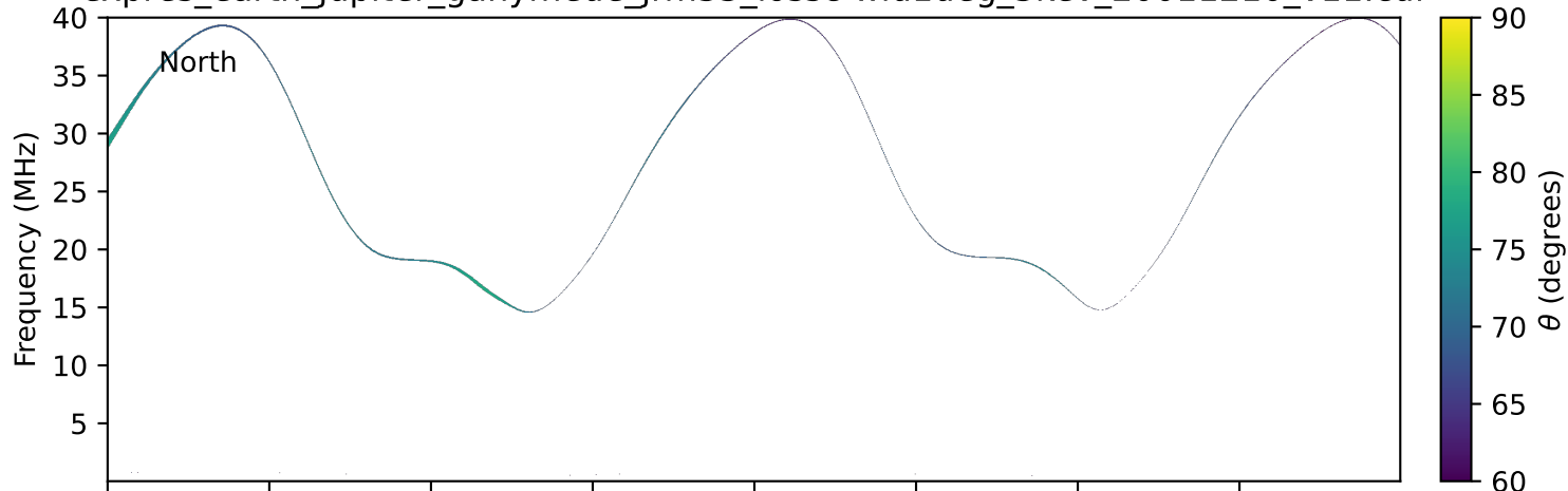
expres_earth_jupiter_ganymede_jrm33_lossc-wid1deg_3kev_20011210_v11.cdf
