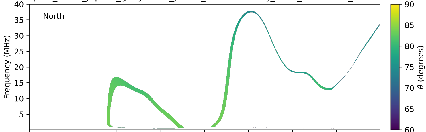
expres_earth_jupiter_ganymede_jrm33_lossc-wid1deg_3kev_20011202_v11.cdf
