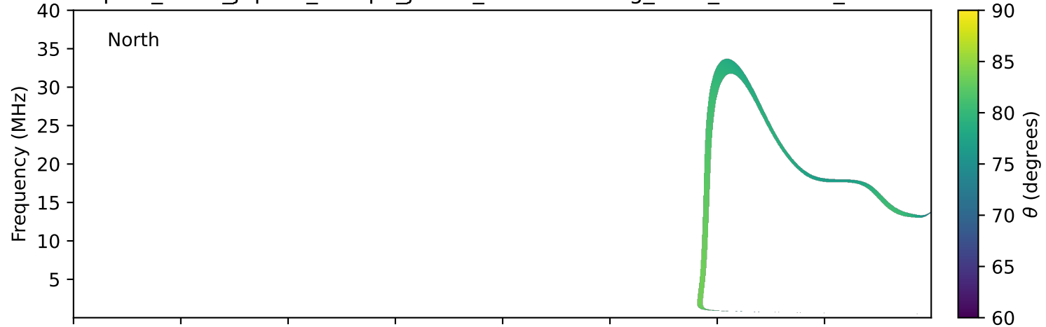
expres_earth_jupiter_europa_jrm33_lossc-wid1deg_3kev_20011218_v11.cdf
