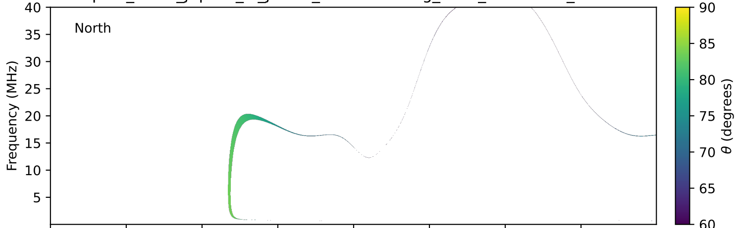
expres_earth_jupiter_io_jrm33_lossc-wid1deg_3kev_20011115_v11.cdf
