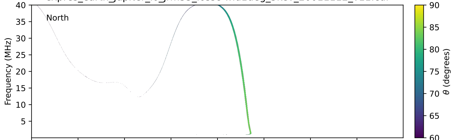
expres_earth_jupiter_io_jrm33_lossc-wid1deg_3kev_20011112_v11.cdf
