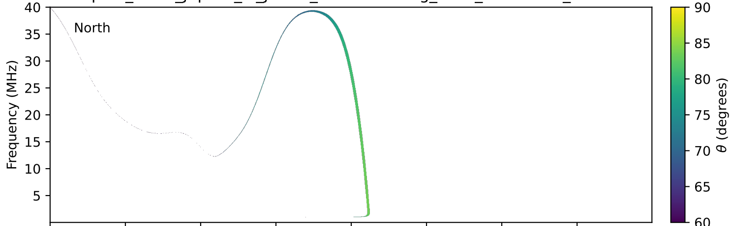
expres_earth_jupiter_io_jrm33_lossc-wid1deg_3kev_20011105_v11.cdf
