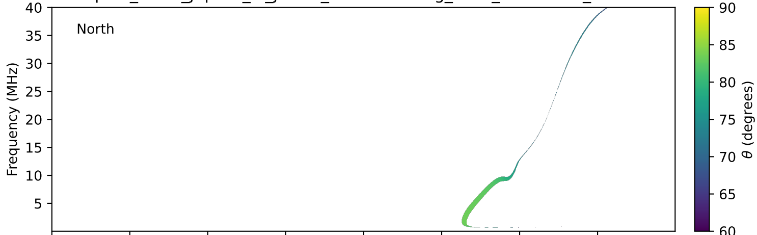
expres_earth_jupiter_io_jrm33_lossc-wid1deg_3kev_20011104_v11.cdf
