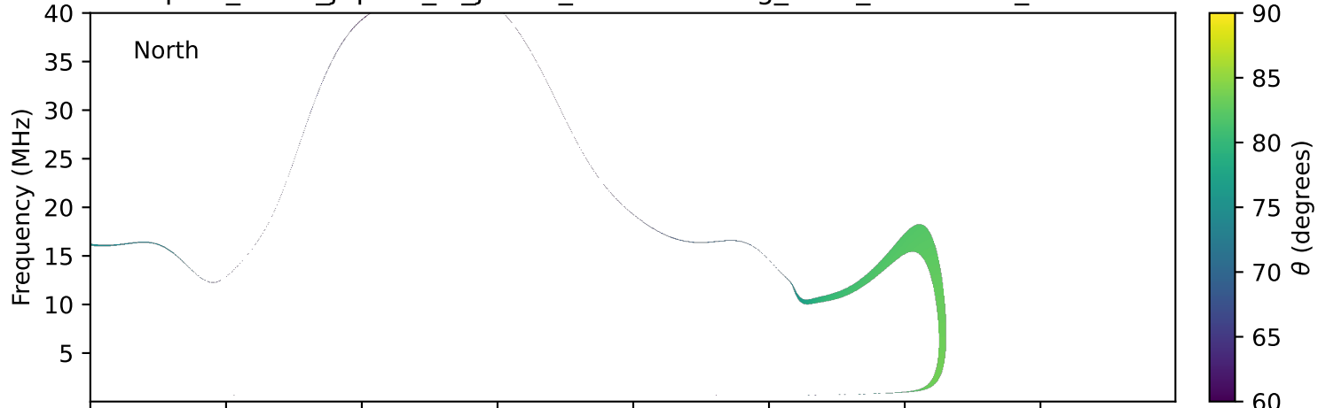
expres_earth_jupiter_io_jrm33_lossc-wid1deg_3kev_20011103_v11.cdf
