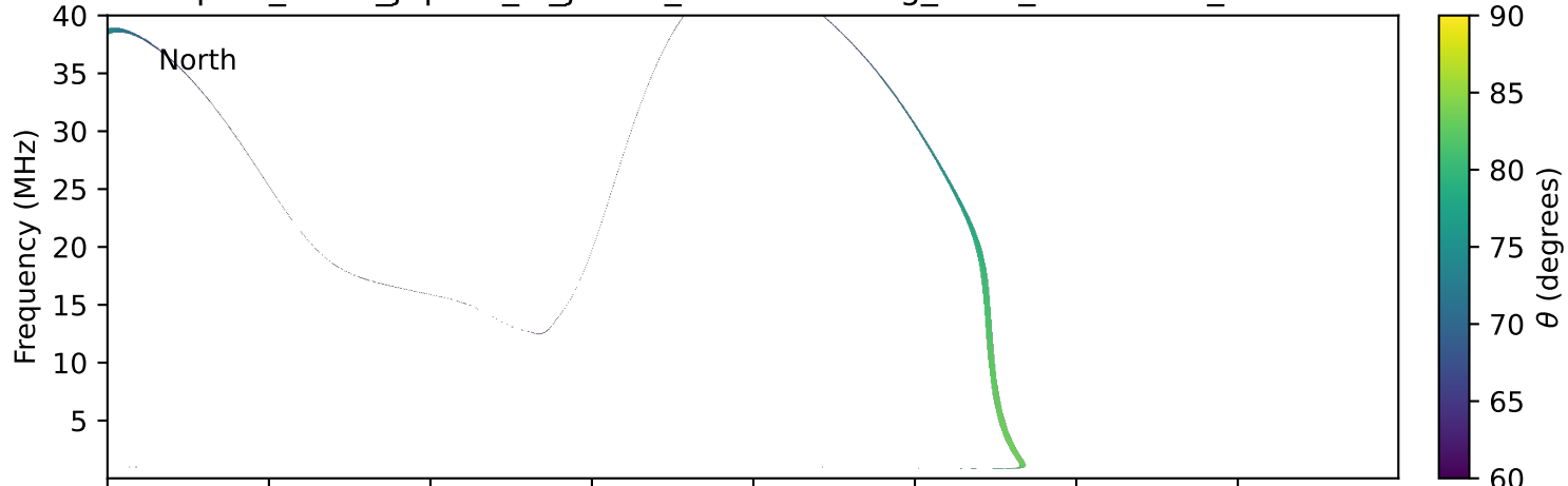
expres_earth_jupiter_io_jrm09_lossc-wid1deg_3kev_20011126_v11.cdf
