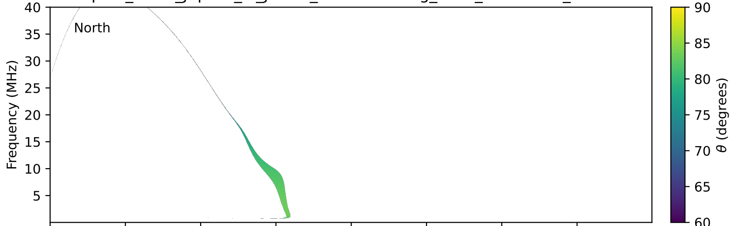
expres_earth_jupiter_io_jrm09_lossc-wid1deg_3kev_20011121_v11.cdf
