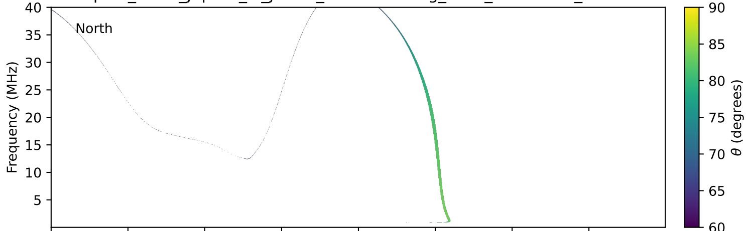
expres_earth_jupiter_io_jrm09_lossc-wid1deg_3kev_20011119_v11.cdf
