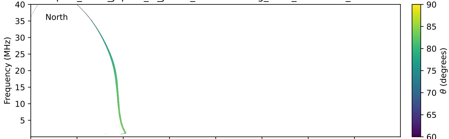
expres_earth_jupiter_io_jrm09_lossc-wid1deg_3kev_20011107_v11.cdf
