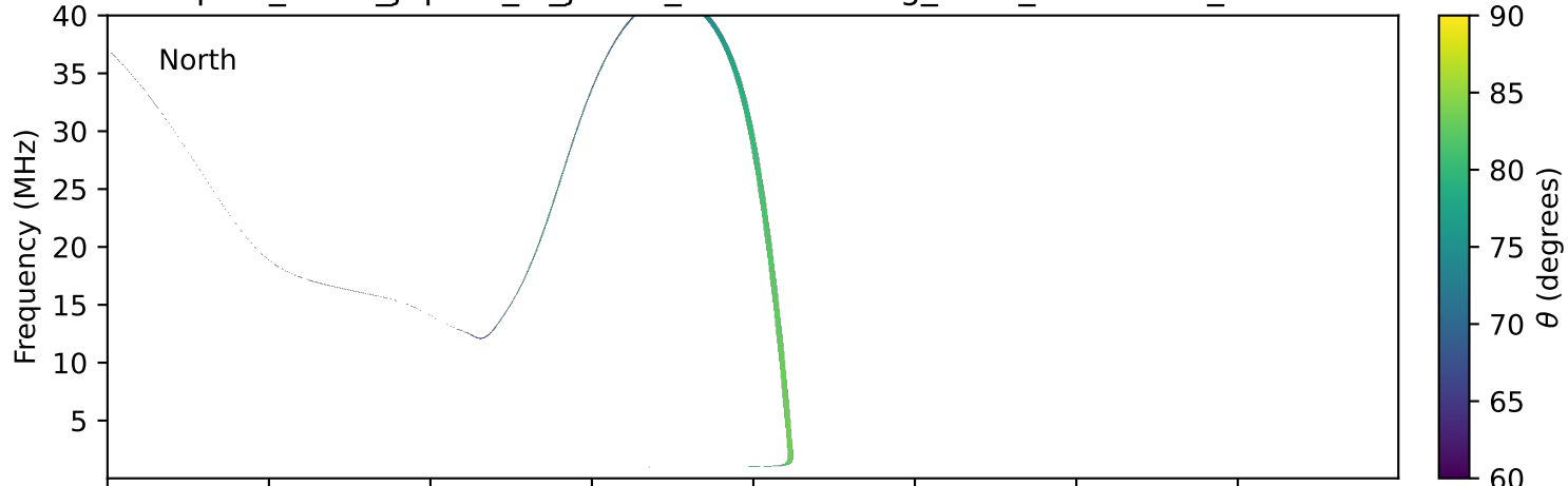
expres_earth_jupiter_io_jrm09_lossc-wid1deg_3kev_20011105_v11.cdf
