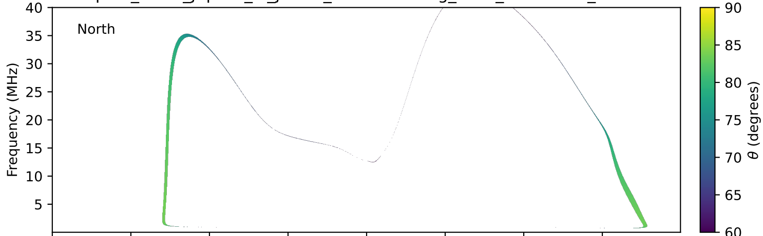
expres_earth_jupiter_io_jrm09_lossc-wid1deg_3kev_20011101_v11.cdf
