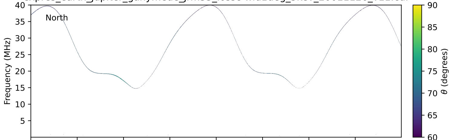
expres_earth_jupiter_ganymede_jrm33_lossc-wid1deg_3kev_20011126_v11.cdf
