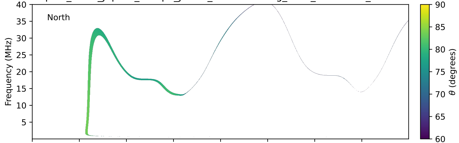
expres_earth_jupiter_europa_jrm33_lossc-wid1deg_3kev_20011106_v11.cdf
